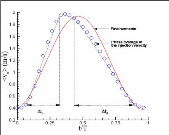
Figure 1 Phase average of the injection velocity.
