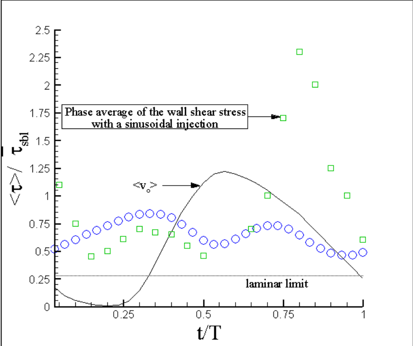
Figure 2 Phase average of the wall shear stress measured at 100 wall units downstream the slot with sinusoidal and dissymmetric blowing velocities oscillating in time.
