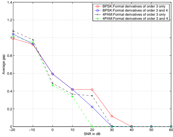
Fig. 3. Gap between estimated and actual mixing matrix for (P, N) = (2, 3) and infinite block lengths; median values over 21 trials of noise are plotted.
