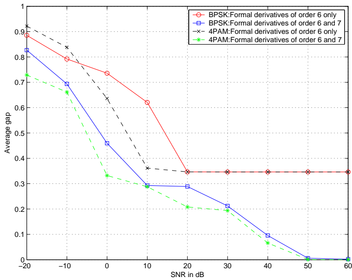
Fig. 4. Gap between estimated and actual mixing matrix for (P, N) = (2, 6) and infinite block lengths; median values over 21 trials of noise are plotted; median values over 21 trials of noise are plotted.
