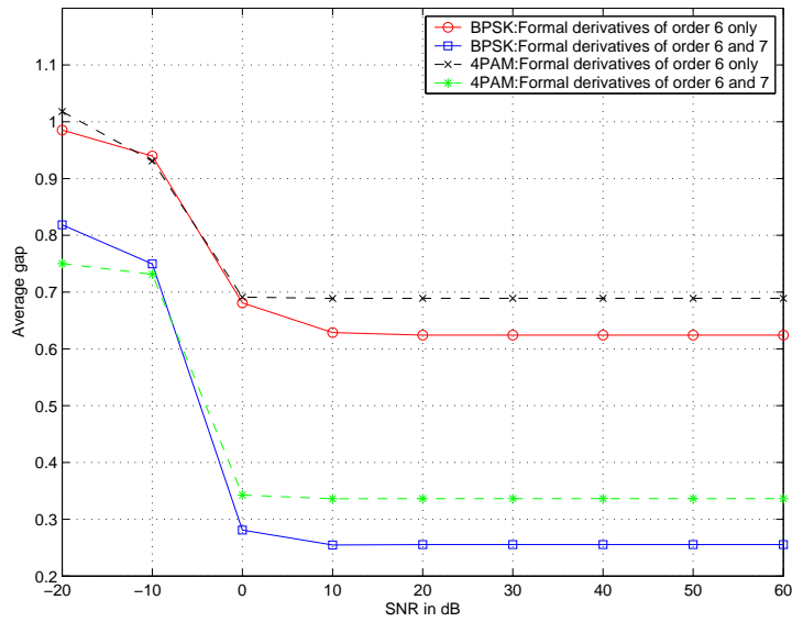
Fig. 2. Gap between estimated and actual mixing matrix for (P, N) = (2, 6) and block lengths of 10000 samples; median values over 21 independent trials of sources and noise are plotted.
