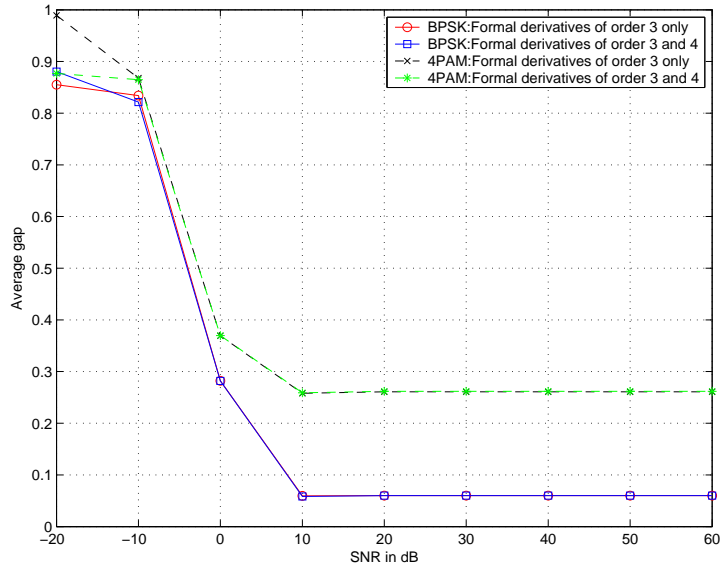
Fig. 1. Gap between estimated and actual mixing matrix for (P, N) = (2, 3) and block lengths of 1000 samples; median values over 31 independent trials of sources and noise are plotted.
