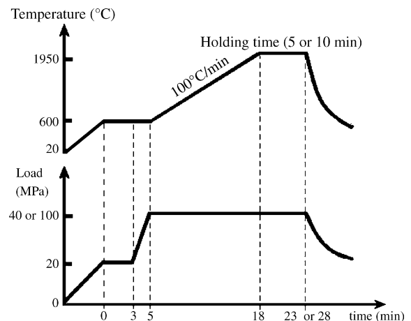
Fig. 1. Thermomechanical cycle applied during the SPS treatment of the ZrC x monoliths and the ZrC x -ZrB 2 composites.
