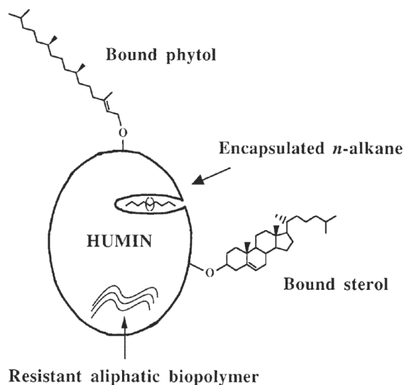
Figure. Model of humin explaining the stabilization of soil organic matter 1) by encapsulation of small polar molecules (physical sequestration), 2) by binding of functionalized biomarkers (chemical sequestration), and 3) by selective preservation of aliphatic biopolymers.
