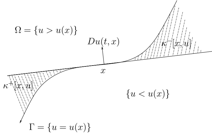
Figure 1: Fractional mean curvature of a curve
