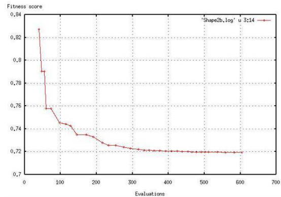
Figure 10 Fitness Convergence (Shape 2)
