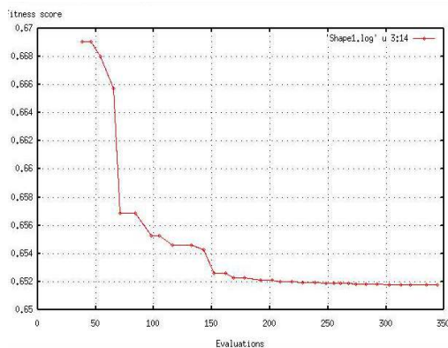
Figure 9 Fitness Convergence (Shape 1)
