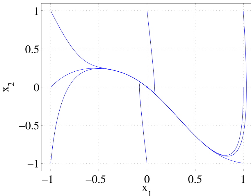
Figure 4: Example 4. Trajectories obtained for r = 10 .
