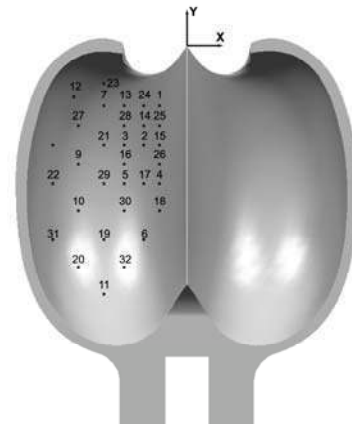
Fig. 3 Transducers's positioning
