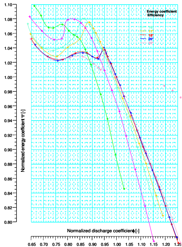
Fig. 10 Pumping Characteristic curves.
