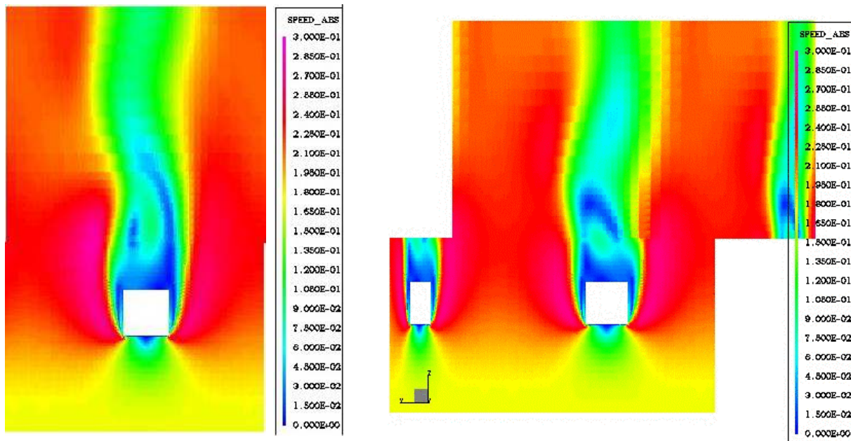
Fig. 7 Flow field for unsteady non R-S computation.
