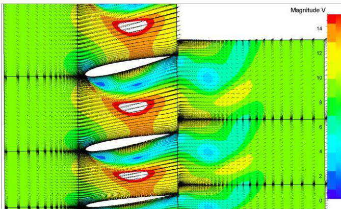
Fig. 3 Large vortex crossing the R-S interface. (Fine Turbo computation)
