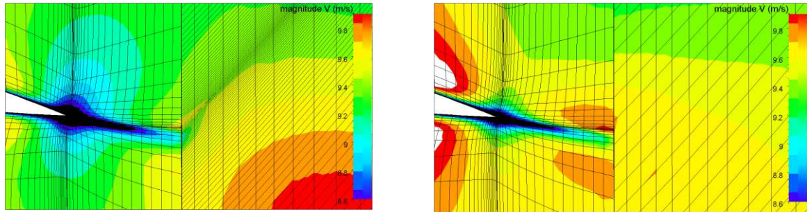
A) The wake crosses R-S through the refined mesh in both sides. B) the wake is diffused by coarse mesh.
