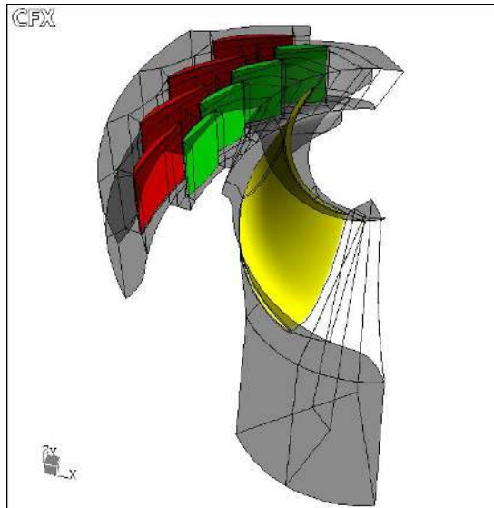
Fig. 11 Pump- turbine computation domain.
