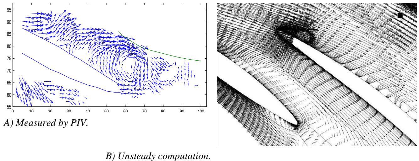
Fig. 18 Instantaneous velocity field near trailing edge of guide vanes at 10% span – Q=0.83Q_n .
