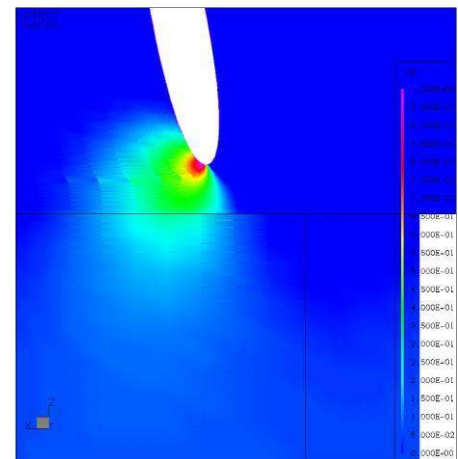
Fig. 4 Upstream pressure perturbation crossing the R-S interface. (Fine Turbo computation)
