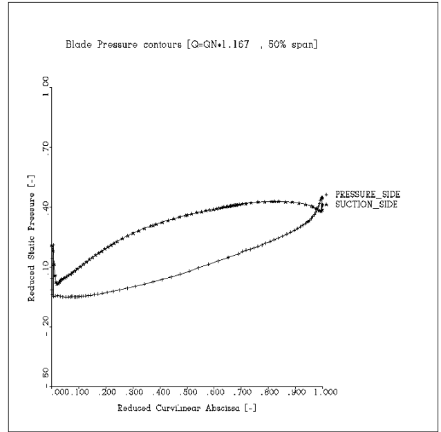
D) Q=1.17Q_n .
