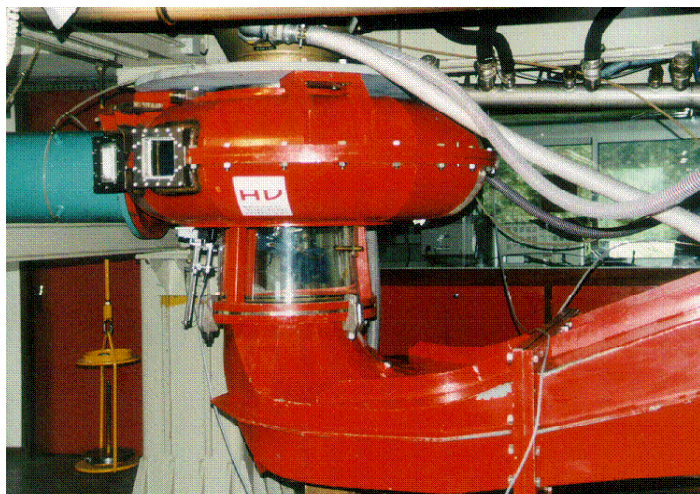
Figure 1 Pump-Turbine model
