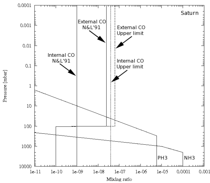
Fig. 4. Ammonia, phosphine and carbon monoxide mixing ratio vertical profiles on Saturn, all in solid lines. The internal and external source of CO models come from Noll & Larson (1991) (N&L'91 on the plot). The upper limits we have derived for the internal source (dotted lines) and for the external source (dashed lines) are also displayed.
