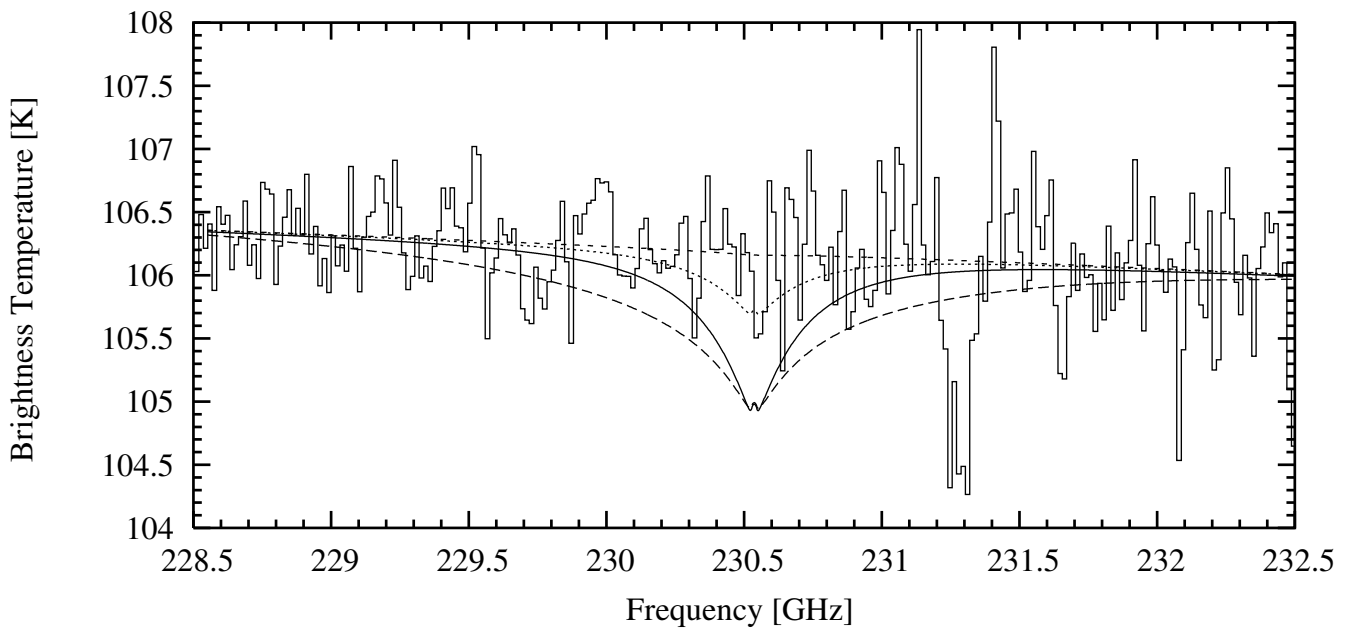
Fig. 6. Observed ^{12}\text{CO} (2-1) spectra on Saturn. The total bandwidth is 4 GHz and the spectral resolution is 16 MHz. The spectra resulting from the upper limits we derived are plotted as follows: our 3\text{-}\sigma upper limit of 6.3 \times 10^{-8} in the stratosphere (external source of CO) in solid line and our 3\text{-}\sigma upper limit of 3.9 \times 10^{-8} constant with altitude (internal source of CO) in long-dashed lines. The internal source of CO model (short-dashed lines) as well as the external source of CO (dotted lines) taken from Noll & Larson (1991) are also plotted for comparison with our upper limits. The absorption feature at 231.280 GHz is the terrestrial \text{O}_3 line.
