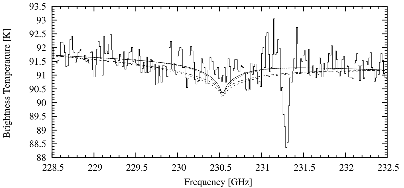
Fig. 7. Observed ^{12}\text{CO} (2-1) spectra on Uranus. The total bandwidth is 4 GHz and the spectral resolution is 16 MHz. The short-dashed lines correspond to the upper limit determined by Encrenaz et al. (2004) for a CO mixing ratio constant with altitude ( q_{\text{CO}} = 2 \times 10^{-8} ). The external source of CO model (dotted lines) is the Encrenaz et al. (2004) best fit model ( q_{\text{CO}} = 3 \times 10^{-8} restricted to the stratosphere). Our 3\text{-}\sigma upper limits are plotted in solid line ( q_{\text{CO}} = 2.7 \times 10^{-8} , restricted to the stratosphere) and in long-dashed lines ( q_{\text{CO}} = 1.8 \times 10^{-8} , constant with altitude). The absorption feature at 231.280 GHz is the terrestrial \text{O}_3 line.
