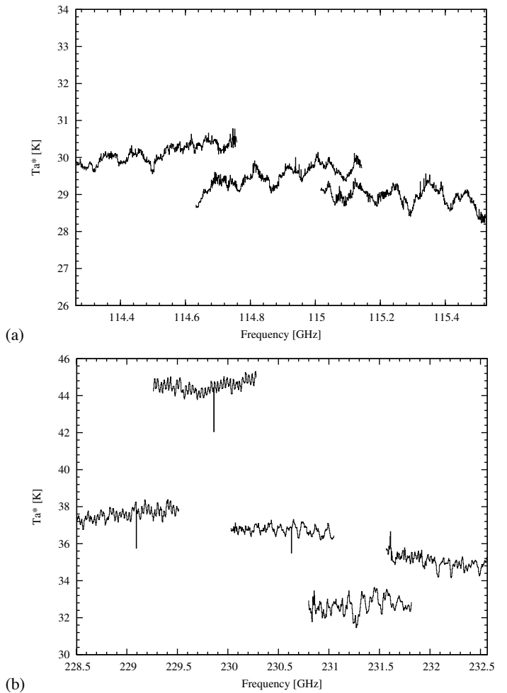
Fig. 1. Spectra of Saturn at (a) 115 GHz and (b) 230 GHz in the antenna temperature scale. Receiver A has a corrupt channel. It can be seen in the middle of the first three lowest frequency bands at 230 GHz. This channel is removed before reducing the spectra. The terrestrial ozone absorption band can be seen at 231.280 GHz. This feature is not taken into account when computing the spectrum noise level.
