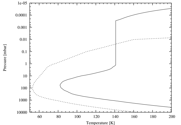
Fig. 3. Thermal profiles of Saturn (solid line) and Uranus (dashed line).
