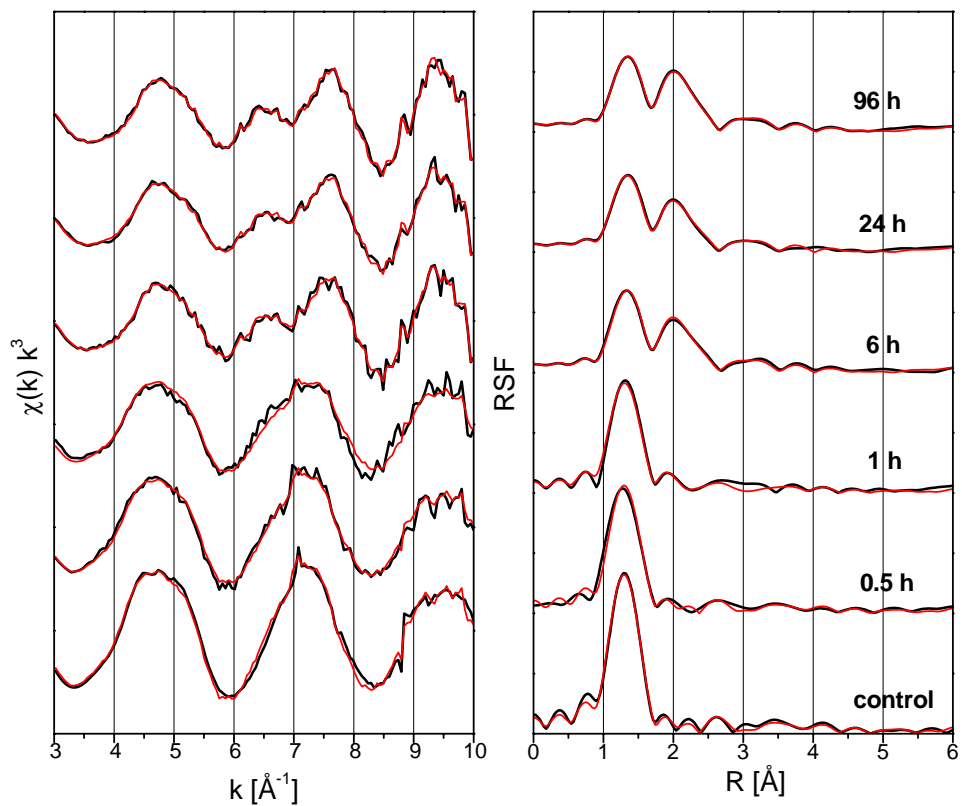
Fig. 10. Se K-edge EXAFS of \text{Fe}^{2+} clays reacted with \text{SeO}_3^{2-} for periods between 0.5 hours and 4 days (black lines). For comparison, the spectra of a \text{Fe}^{2+} -free control (bottom) is shown. Red lines represent the reconstruction of the spectra with 2 components, extracted from the 6 clay spectra by ITFA.
