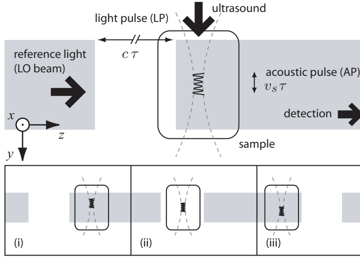
Figure 2. Stroboscopic detection of the acoustic pulse AP (pulse length v_s\tau where v_s \simeq 1500m/s is sound velocity) by the LO beam light pulse LP (pulse length c\tau where c is light velocity). (i) the AP propagates in the sample while the LO beam is turned off. (ii) AP and LP overlap within the AO volume of interest. Heterodyne amplification and detection of ultrasound-tagged photons occurs. (iii) the LO beam is turned off until the next AP reaches the AO volume.
