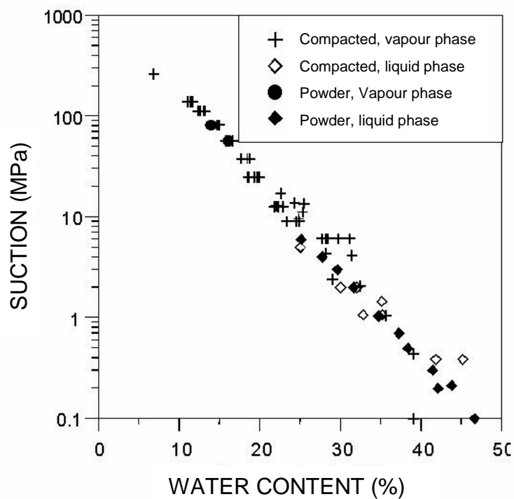
Figure 28 : Water retention properties of an engineered barrier FoCa7 clay (Yahia-Aissa et al. 2000)
