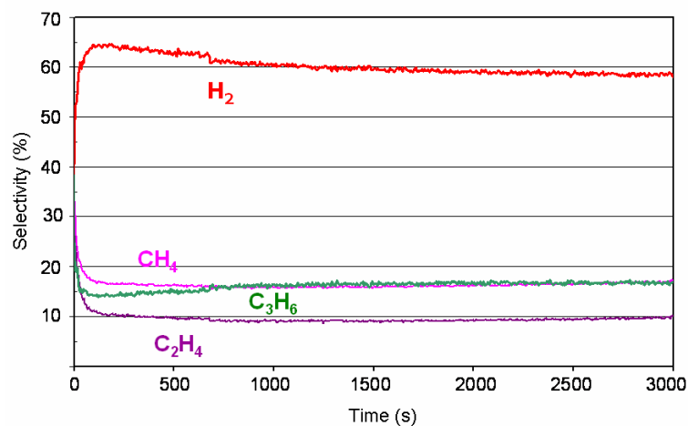
Figure 3: Selectivity to products vs. time using a BICOVOX membrane covered with BICOVOX/Au cermet at OCV (700°C, 1% C_3H_8 /He in LOP, air in HOP).
