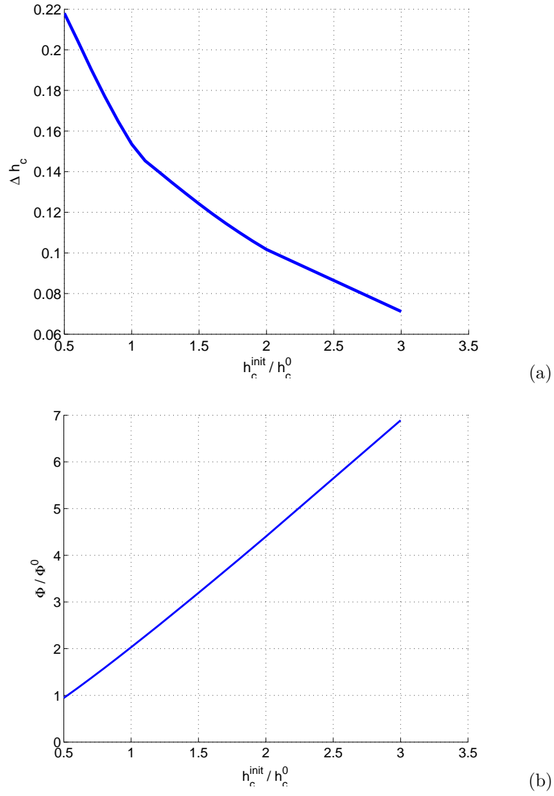
Fig. 14. Influence of the initial constriction height h_c on the partial closure of the channel (a) and on the flow rate (b). Simulations with parameters : \Delta P = 150 Pa, P_{\text{ext}} = 200 Pa, E = 1.6 MPa.
