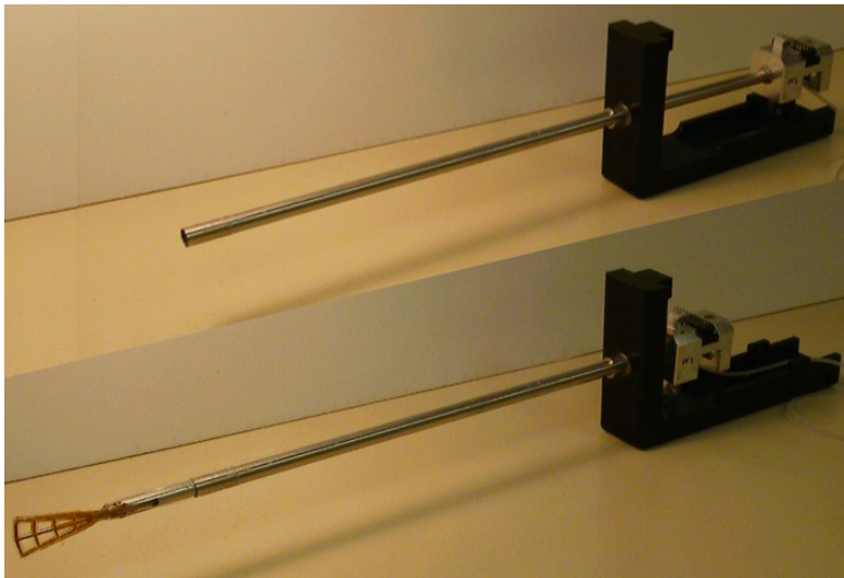
Figure 5: retracted/deployed umbrella.
