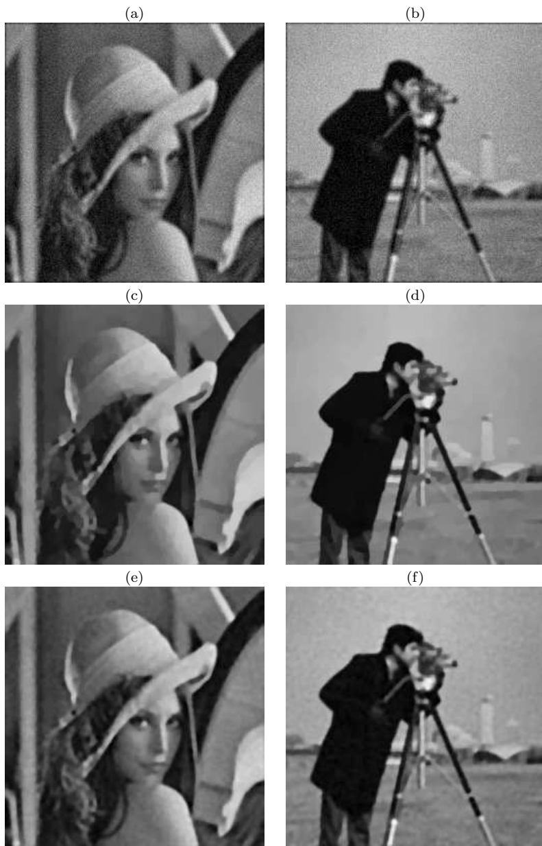
Figure 3: (a) and (b) : degraded images (convolved with a Gaussian kernel with standard deviation \eta = 5 , and then degraded by a zero mean Gaussian noise with standard deviation \sigma = 10 ), the original images are on top row of Figure 1; (c) and (d) : total variation restoration with schemes (75) and (24), with \lambda = 5 ; (e) and (f) : smoothed total variation based restoration with schemes (75) and (43), with \lambda = 5 and \beta = 10 .
