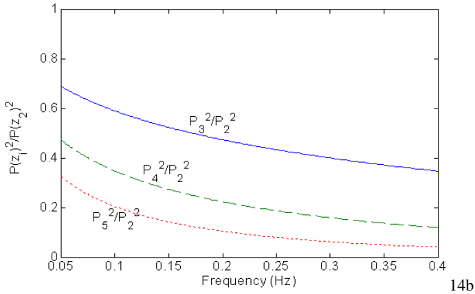
Figures 14a & 14b: Variations with frequency of the damping coefficient of pressure variations at three different levels inside the soil, experimental & predicted by Sakai's equations.
