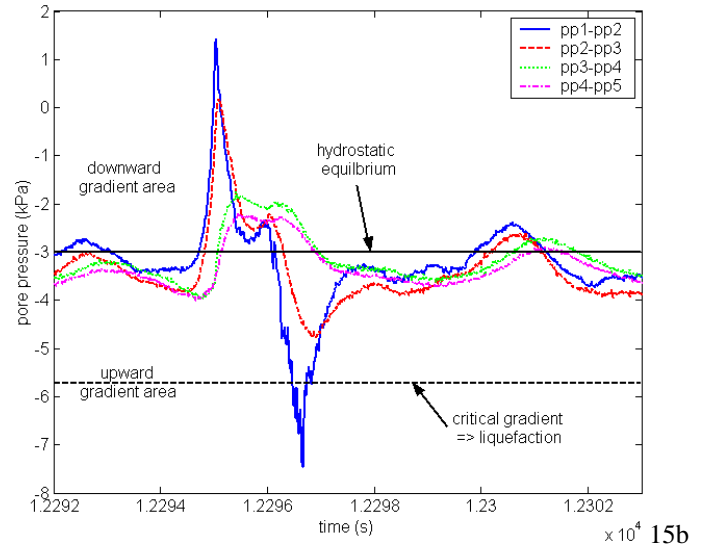
Figure 15a & 15b. Pore pressure transducers response at the time scale of a wave. An example of a liquefaction event.
