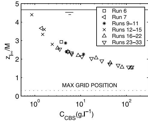
Figure 5. Variation in lutocline position with mean CBS layer concentration. The grid frequency is F = 4 Hz. Symbols and experimental parameters are given in Table 1.
