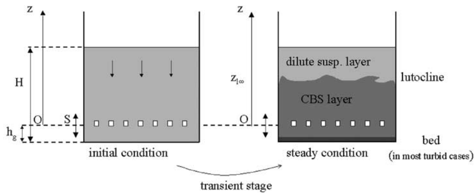
Figure 3. Grid-stirred experimental procedure.
