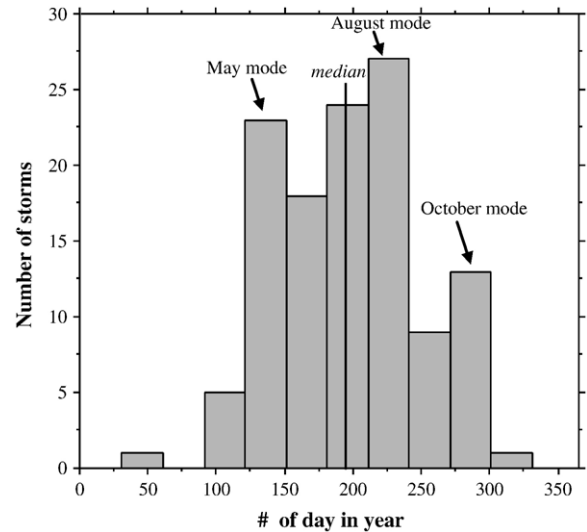
Fig. 2. High-intensity rainfall events recorded between 1992 and 2001 in the Vosne-Romanée vineyards.
