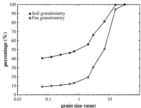
Fig. 8. Grain-size distribution in reference soil sample and in fan.
