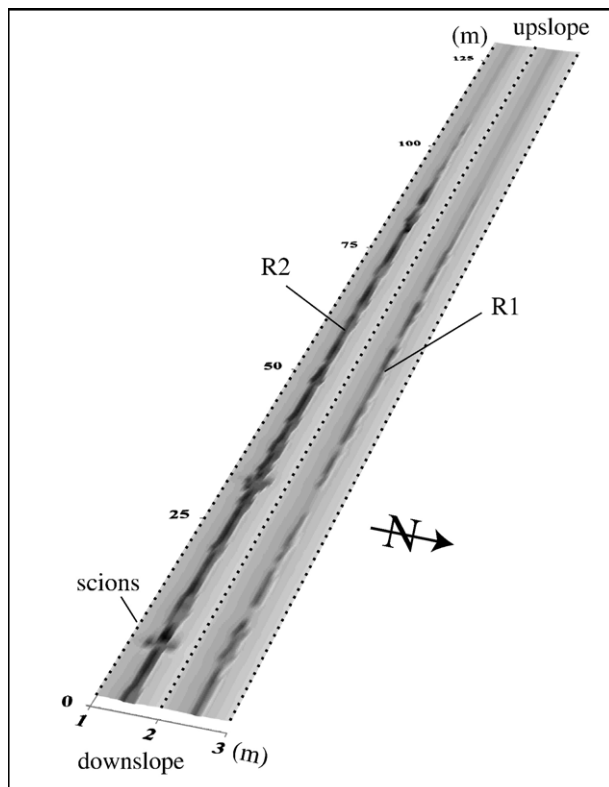
Fig. 5. Digital reconstruction of the R1 and R2 rill system, used to assess rill volume.
