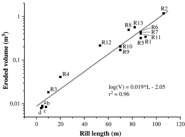
Fig. 7. Relationship between eroded volume and rill length.
