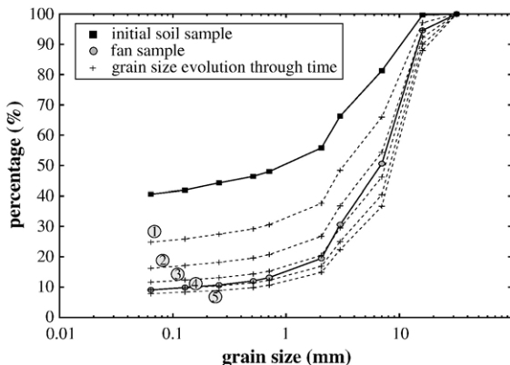
Fig. 9. Simulation showing temporal evolution of grain-size distribution in soil for five successive events.
