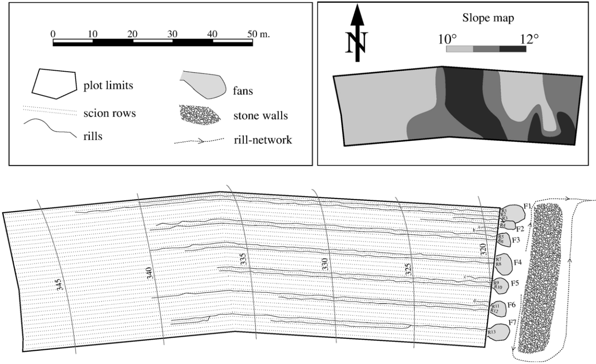
Fig. 3. Slope and plot map showing the regularly spaced rills and the associated fans. The major rills are numbered from 1 to 13, the fans from 1 to 7.
