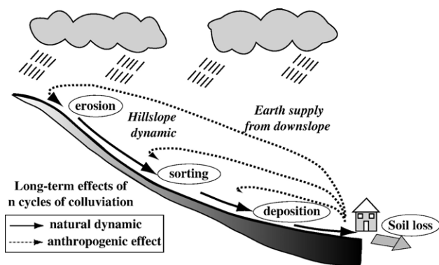
Fig. 1. Hillslope dynamics resulting from the interaction between natural and anthropogenic processes in a vineyard context.
