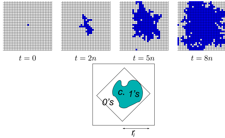
FIGURE 3 Top : Example of a simulation for rule \mathbb{T}62 . Bottom : Schematic view of a configuration where a region of 1's reaches the sphere \partial(c, r_i) .
