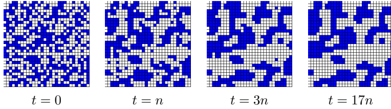
FIGURE 2 Example of a simulation for rule \mathbb{T}56 , when \sigma^0 is a random uniform configuration.
