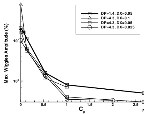
Fig. 4. Maximum normalized wobble amplitude in % in terms of C_\mu for the 1D stationary shock wave.
