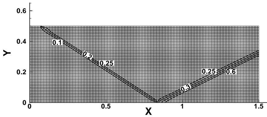
Fig. 17. The interaction of an oblique shock with an inviscid wall. The shock angle is 33 degrees from the Mach 3 free-stream. Contours of normalized pressure are plotted.
