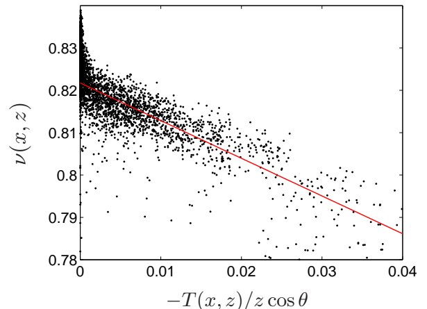
Fig. 4. Time and ensemble averaged volume fraction \nu(x, z) as a function of the ratio T(x, z) / z \cos \theta for \Omega = 6 rpm. For this rotation speed, the mean slope of the free surface was measured to be \theta \simeq 19.7^\circ [27]. The straight line is a fit given by equation (23) with K \simeq 1.1 and \nu_* \simeq 0.822 . The temperature is non-dimensionalized by gd where g refers to the gravity constant and d to the mean diameter of the beads (see text for details).
