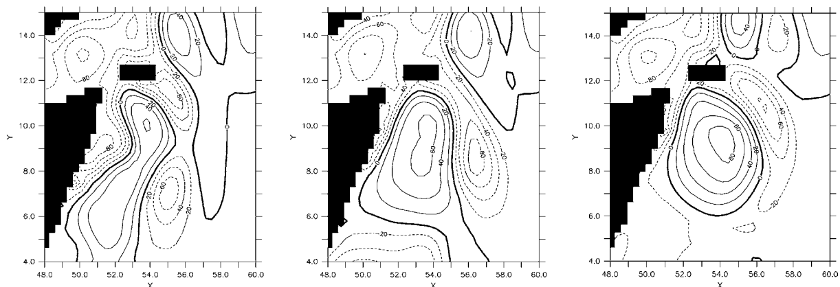
Fig. 7. Layer thickness anomalies (in m) relative to 10-year mean of all months at 3 consecutive August 1 in the low-friction experiment RG-lo95.
