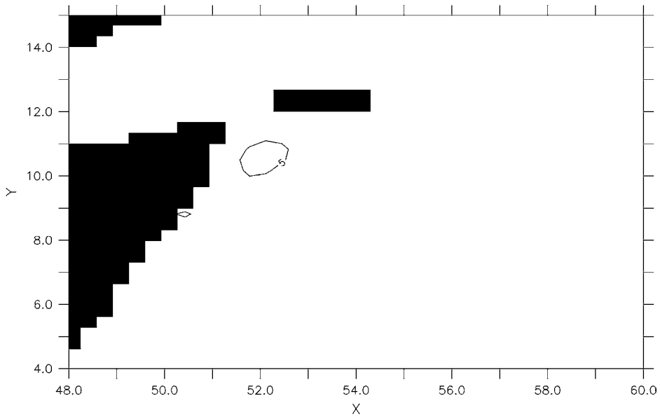
Fig. 9. As Fig. 8, but for the high-viscosity experiments RG-hi.
