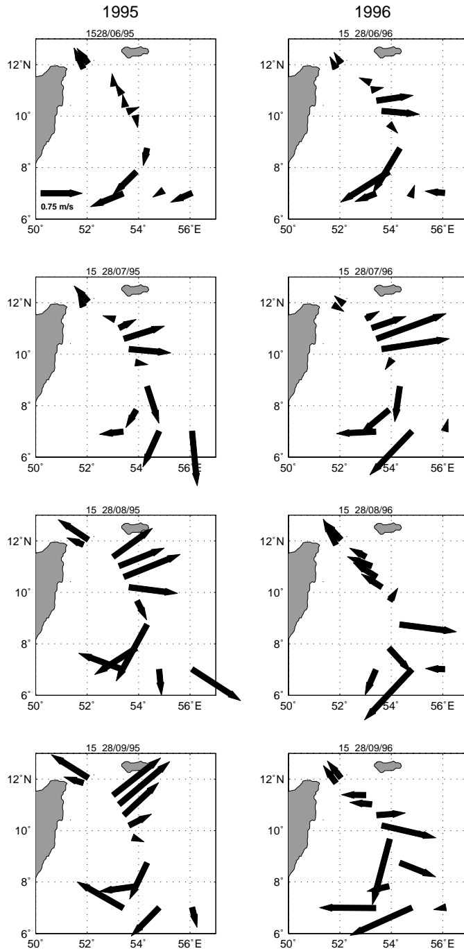
Fig. 2. Time series of near-surface current vector plots from the Great Whirl and Socotra Passage region (15 day means) for June–September (a) 1995, (b) 1996. Note the differences in GW intensities of both years and that the 1996 GW collapsed much earlier (from Schott and McCreary, 2001).
