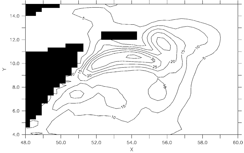
Fig. 8. Standard deviation due to external (upper) and internal (lower) variability for the low-viscosity exps. RG-lo (contour interval is 5 m). The standard deviation due to the external part is calculated using the variance of the means over 10 realizations for each of the years 1993, 1995 and 1996. The standard deviation of the internal part is calculated using the average variance for the years 1993, 1995 and 1996.
