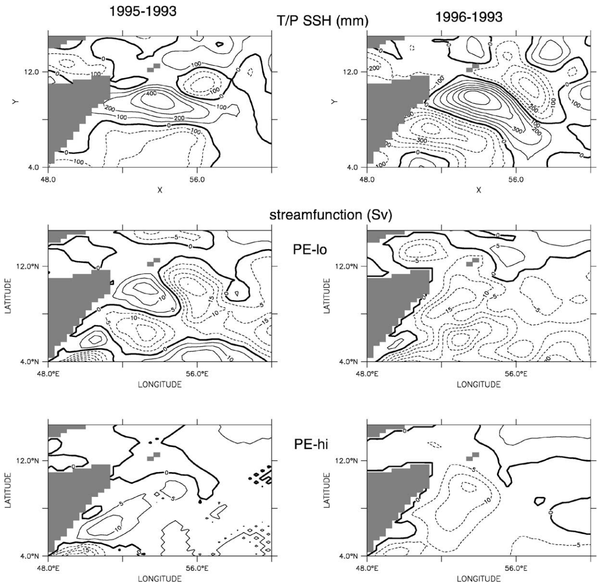
Fig. 6. Interannual variability of the GW on August 1. Left panels show values for 1995 minus 1993, right panels 1996 minus 1993. Top panels gives SSH from Topex/Poseidon (in mm), middle and bottom panels show depth integrated transport stream function from exp. PE-lo (middle) and PE-hi (bottom), both in Sv.
