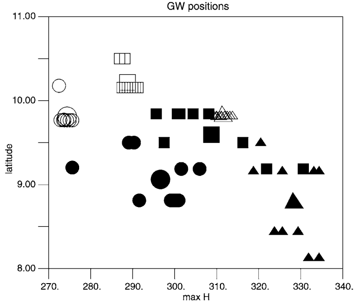
Fig. 10. Mean layer thickness vs. meridional position of the GW in the different experiments with the RG model. Triangles, squares and circles correspond to exps. with forcings of the years 1993, 1995 and 1996, respectively; solid and open symbols are for low and high-friction experiments, respectively; large symbols represent the mean values.
