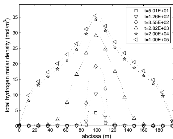
Fig. 4 Test case 2 : spatial evolution along the line \mathcal{L}_{cut} of the total hydrogen molar density \frac{\rho_g^{sd}}{M^h} X at several times t (in years)
