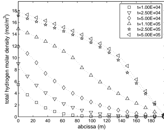
Fig. 1 Test case 1 : spatial evolution along the line \mathcal{L}_{cut} of the total hydrogen molar density \frac{\rho_k^{st}}{M^h} X at several times t (in years)
