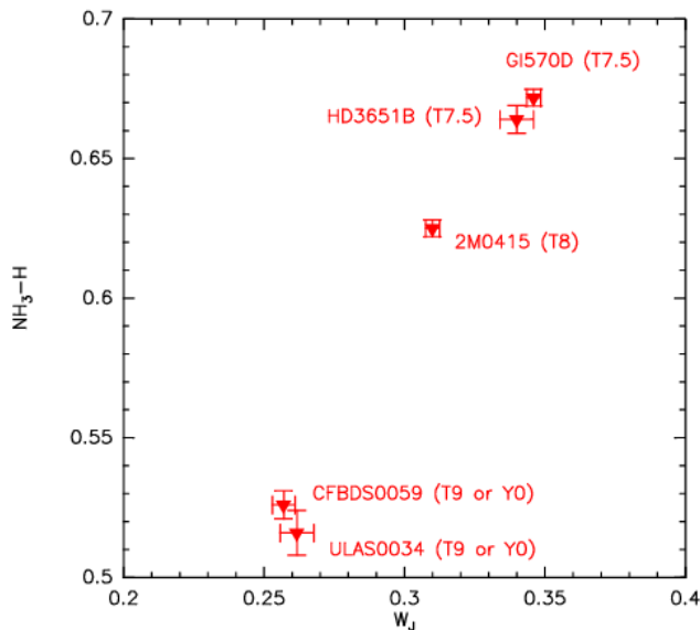
Fig. 11. NH 3 - H index versus W_J index. The error bars represent the 1\sigma uncertainties of the measured spectral indices.
