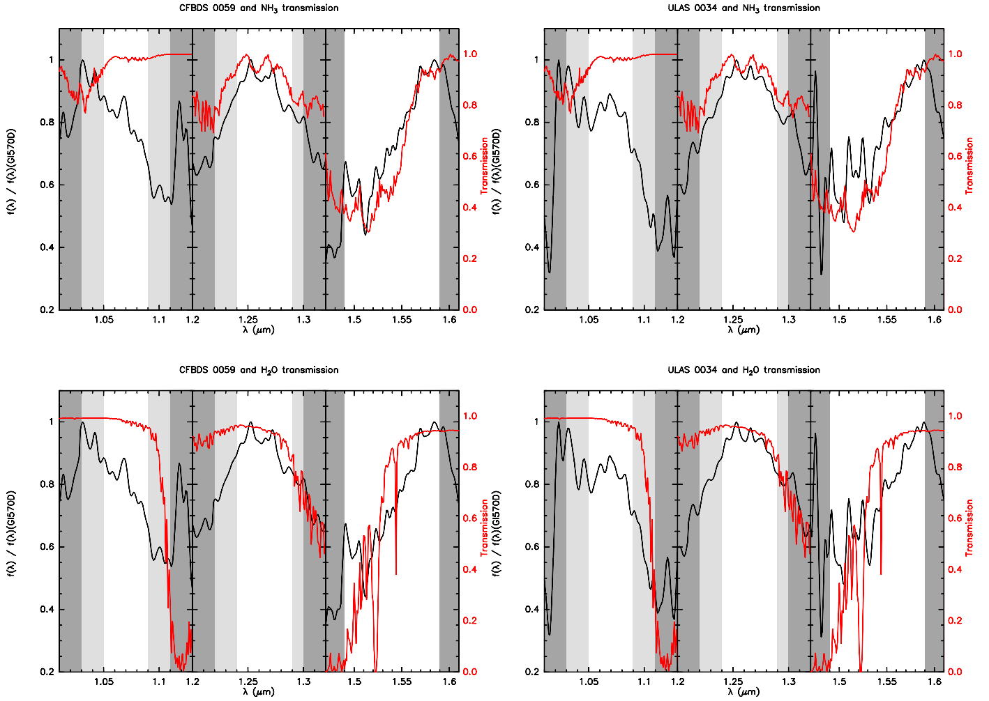
Fig. 9. Flux ratio between CFBDS0059 and GI 570D (black), together with the laboratory room temperature transmission spectrum of NH 3 (Irwin et al. 1999) (red, top panel) and the 600 K H 2 O transmission spectrum computed from the HITRAN molecular database (red, bottom panel). The grey bands mark the parts of the spectrum affected by strong (dark grey) or moderate (light grey) CH 4 absorption.
