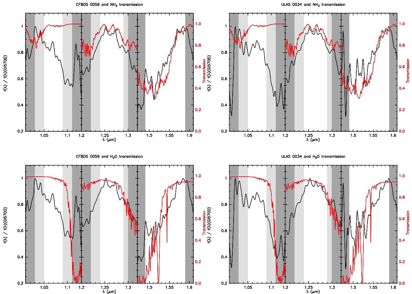
Fig. 9. Flux ratio between CFBDS0059 and Gl 570D (black), together with the laboratory room temperature transmission spectrum of \text{NH}_3 (Irwin et al. 1999) (red, top panel) and the 600 K \text{H}_2\text{O} transmission spectrum computed from the HITRAN molecular database (red, bottom panel). The grey bands mark the parts of the spectrum affected by strong (dark grey) or moderate (light grey) \text{CH}_4 absorption.
