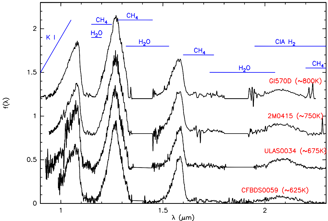
Fig. 4. 0.9 \mu\text{m} - 2.3 \mu\text{m} spectra of CFBDS0059 and the three other coolest brown dwarfs. The spectra are normalized to unit flux densities at their 1.27 \mu\text{m} .peak, and vertically offset for clarity. The main T-dwarf spectral features are labeled. The temperatures of GI 570D and 2M0415 are from the careful spectroscopic analyses of Saumon et al. (2006) and Saumon et al. (2007). Those of CFBDS0059 and ULAS0034 are from our W_J versus J/K index (Fig. 6).
