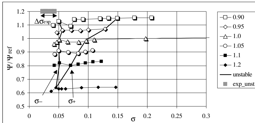
Figure 16. Efect of the flow rate on the cavitation characteristic and on the instability range (comparison with the experimental instability range in grey)
