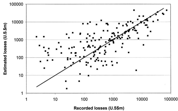
FIG. 8. Each point represents a historical hurricane landfall. The abscissa is the recorded normalized economic losses due to landfall. The ordinate is the normalized economic losses estimated from the maximum wind speed at landfall and the estimated local vulnerability. Both axes are in logarithmic scales.
