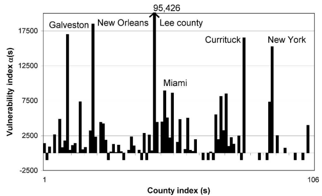
FIG. 7. Historical local vulnerability coefficients, county per county. The negative bars represent the counties for which no data are available.
