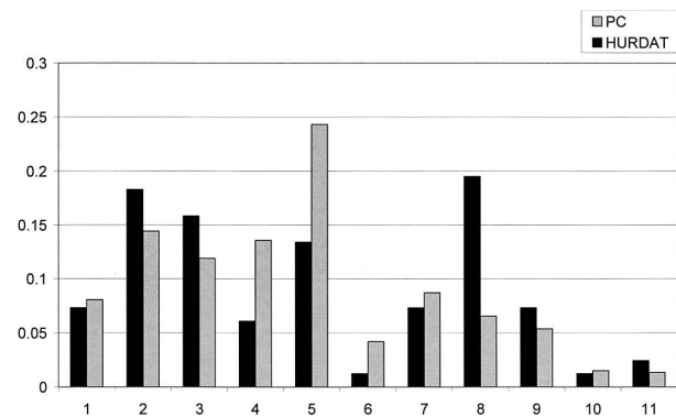
FIG. 5. Distribution of hurricane landfalls for each of the 11 regions, estimated from HURDAT and from synthetic tracks for the PC.
