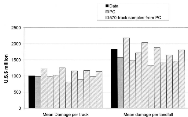
FIG. 9. Mean damage per track and per landfall from historical data, from synthetic tracks generated for the present climate, and from the ten 570-track samples extracted from the PC synthetic tracks.
