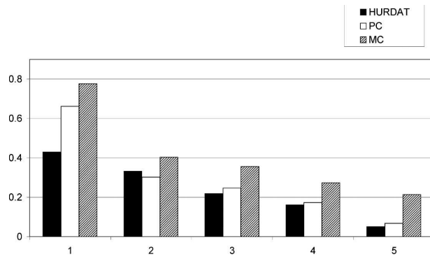
FIG. 2. Annual probability of landfall of a hurricane of a given category, estimated from HURDAT and from synthetic tracks for the PC and MC.
