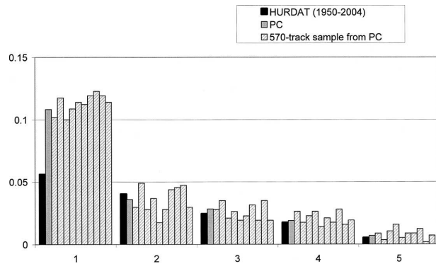
FIG. 3. Same as in Fig. 1, but from HURDAT, the synthetic tracks in PC, and 10 samples of 570 synthetic tracks.
