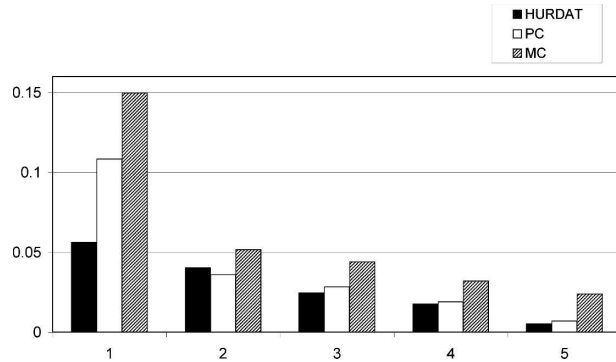
FIG. 1. Probability, for a given storm, of making landfall as a hurricane of categories 1–5, estimated from HURDAT and from synthetic tracks for the PC and an MC.
