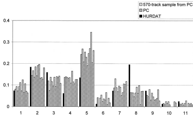
FIG. 6. Distribution of hurricane landfalls in each region, estimated from historical data, from the synthetic tracks for the present climate and from 10 samples of 570 tracks.
