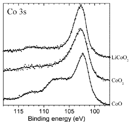
Figure 6. Co 3s core peaks of LiCoO 2 , CoO 2 , and CoO.
