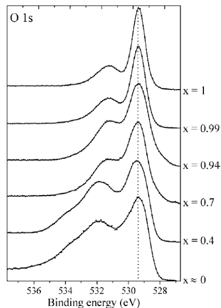
Figure 7. O 1s core peaks of Li x CoO 2 ( 0 \leq x \leq 1 ).
