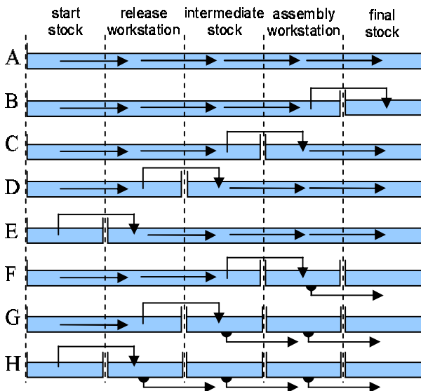
Fig. 4. Architectures Which Contain a Maximum of One Transfer Through the Air.
