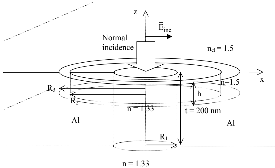
Fig.1. Schematic representation of a screen with a circular aperture and a circular channel around it, made in an aluminum screen with thickness t = 200 \text{ nm} . The cladding is glass and the substrate is water. The channel width is R_3 - R_2 , its depth h , and it is filled with glass.
