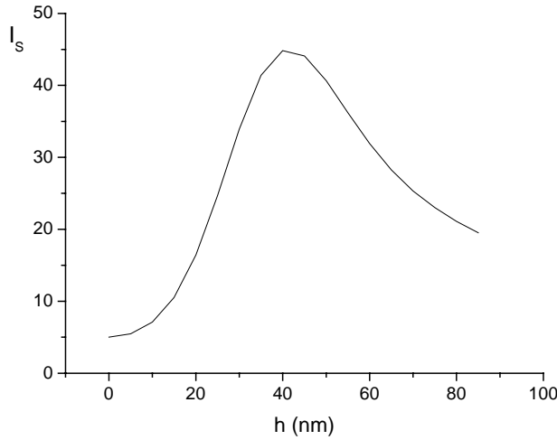
Fig.2. Field enhancement averaged in a plane z = -5 nm inside the aperture as a function of the channel depth h for R_1 = 75 nm, R_2 = 200 nm, R_3 = 280 nm.
