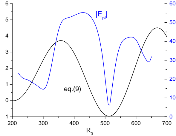
Fig.7. Absolute value of the electric field amplitude of the plasmon surface wave (in blue) as a function of R_3 when R_2 = 200 nm and n_{cl} = 1.5 , compared with the coupling between the incident light and the plasmon, as given in eq.(9)
