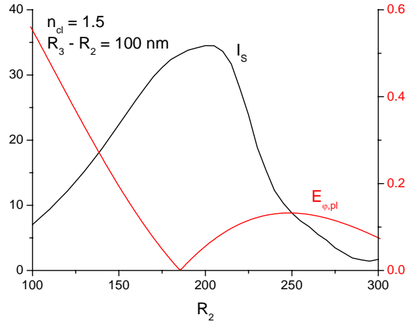
Fig.5. Comparison of the position in R_2 of the maximum of the enhancement factor I_s with the minimum of the surface plasmon electric field components tangential to the channel wall
