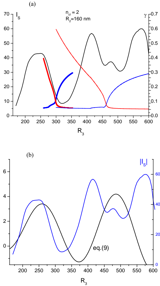
Fig.8. Response (as in Figs.4 and 7) as a function of R_3 of the structure with cladding index n_{cl} = 2 and R_2 = 160 nm. (a) I_s and \gamma , (b) incident wave – surface plasmon coupling integral according to eq.(9).
