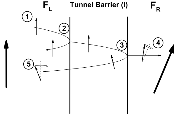
Figure 7: Schematics of the principle of spin transport in a magnetic trilayer with non collinear electrodes magnetizations. Step 1: the electron spin is polarized along the magnetization of the left electrode. Step 2: After the first reflection/transmission by F_L/I interface the reflected and transmitted parts remain in a pure spin state. Step 3: The reflection/transmission by the second interface I/F_R reorients the electron spin. Step 4 and 5: The transmitted and reflected spins precess around the local magnetization.
