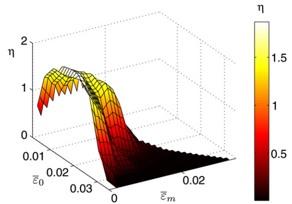
Figure 31. Loss factor: \eta versus (\bar{\varepsilon}_0, \bar{\varepsilon}_m) represented in three dimensions.
