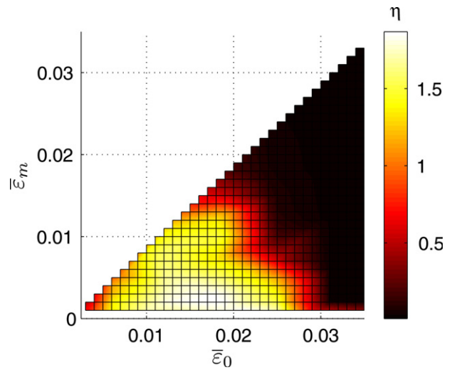
Figure 30. Loss factor: \eta versus (\bar{\varepsilon}_0, \bar{\varepsilon}_m) .
