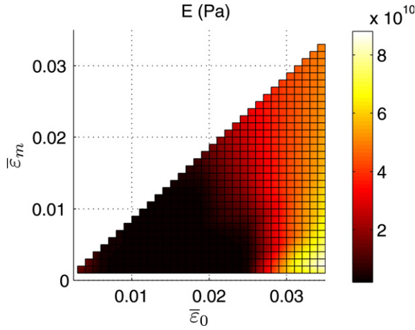
Figure 28. Storage modulus: E versus (\bar{\epsilon}_0, \bar{\epsilon}_m) .
