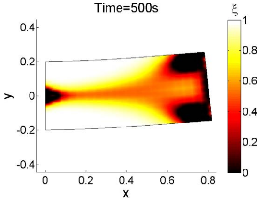
Figure 15. \xi at t = 500 s.
