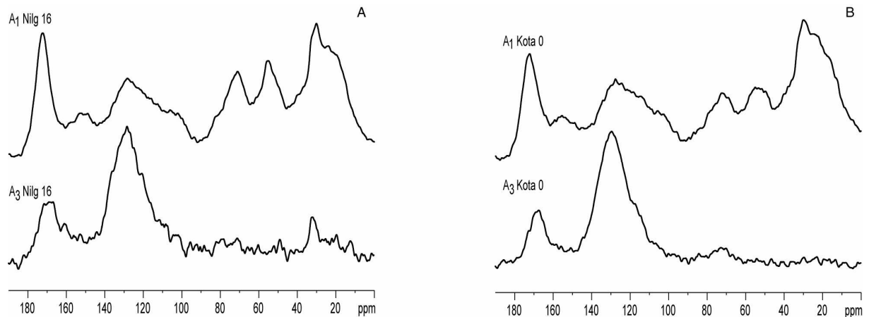
Figure 4: Solid state 13 C-NMR spectra of humic acids from the Nilg 16 (A) and Kota 0 (B) pedons (A 1 and A 3 horizons).
