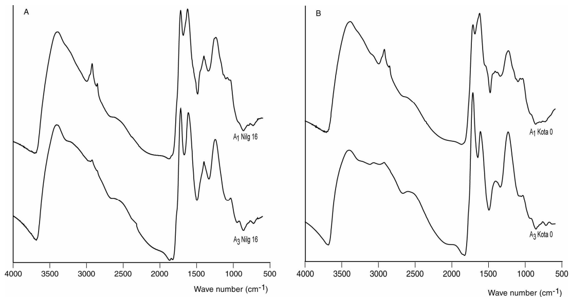
Figure 3: FT-IR spectra of humic acids from the Nilg 16 (A) and Kota 0 (B) pedons (A 1 and A 3 horizons).
