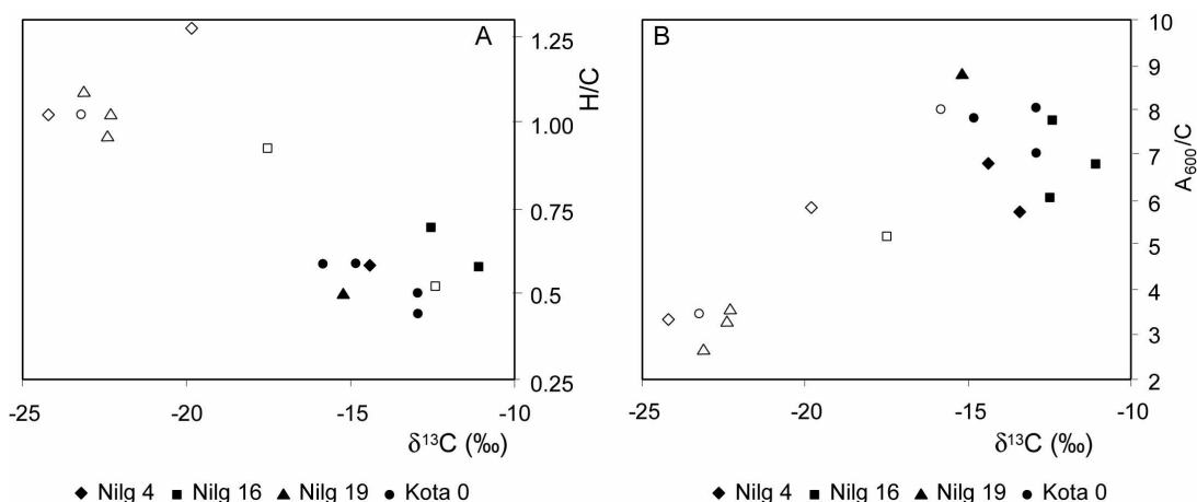
Figure 5: Plots of H/C ratios (A) and colour intensity values (B) of HAs versus the SOM \delta^{13}\text{C} values. Samples having \delta^{13}\text{C} values higher than -15\text{‰} and aromatic and melanic HAs are part of a population that is statistically different from the one that includes the other samples. Filled symbols correspond to SOM from subsurface horizons having a Munsell colour of 5YR 2.5/2, whereas open symbols correspond to SOM from horizons having a Munsell colour lighter than 5YR 2.5/2.
