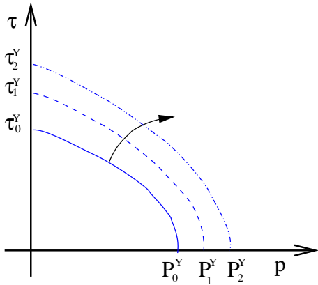
FIG. 3: Limit of the elastic domain in the space of stresses (pressure in abscissa, equivalent shear stress in ordinate). The behavior remains elastic for any stress left or below this limit. When stress reaches this limit, plasticity sets in and the limit curve can be convected at higher stresses (hardening). Pressure cycles allow to give a quantitative account of the evolu-
