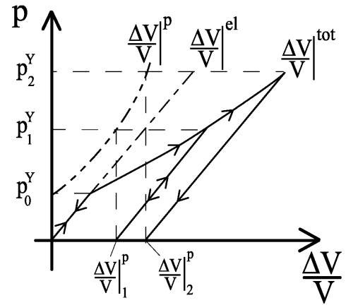
FIG. 2: Sketch of a typical pressure/density curve expected in elastoplasticity. A reversible elastic behavior is obtained up to the elastic limit pressure P_0^Y . When loading above P_0^Y , plasticity sets in and the (elastic) unloading from P_1^Y is characterized by a residual densification. A subsequent loading at P_2^Y > P_1^Y reproduces the previous unloading curve up to P_1^Y before plasticity sets in again. The elastic limit has thus evolved under loading from P_0^Y to P_1^Y and P_2^Y . The knowledge of this density hardening behavior (evolution of the limit elastic pressure with density at zero pressure) is necessary to give a proper modelling of plasticity of glasses.
