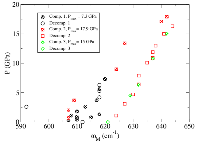
FIG. 5: Raman shift of D_2 line \omega_{D2} in the elastic-plastic regime (same conditions as above).
