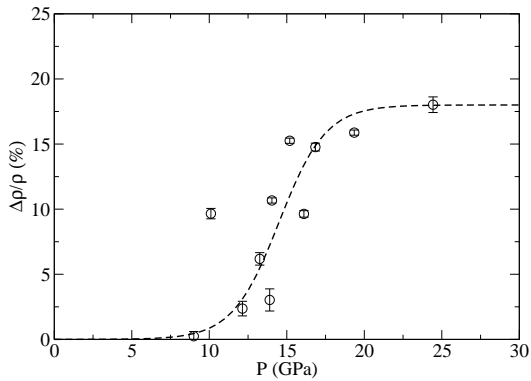
FIG. 6: Evolution of the residual densification vs the maximum pressure of the pressure cycle (symbols). The dashed line is an indicative sigmoidal curve corresponding to a 18% maximum densification.
