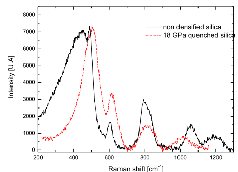
FIG. 1: Raman spectra obtain with an amorphous silica sample before (plain line) and after (dotted line) a 18 GPa hydrostatic loading.
