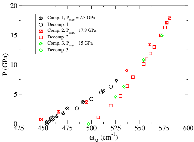
FIG. 4: Raman shift of the main band \omega_M in the elastic-plastic regime. Successive pressure loading and unloading cycles are depicted. Filled and empty symbols correspond to loading and unloading curves respectively. For a pressure maximum P_{max} = 7.3 GPa, a full reversibility is obtained (elastic behavior). For a larger maximum pressure P_{max} = 18 GPa, a residual shift is obtained after unloading (plastic behavior). An additional loading at P_{max} = 16 GPa reproduces the last unloading curve, indicating the increase of the elastic limit under loading (hardening).
