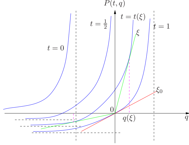
Figure 3. Solution of (4.11)
