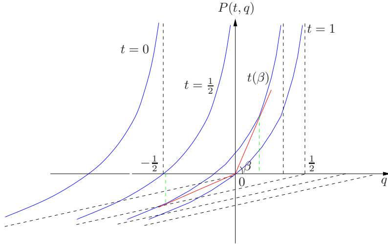
Figure 4. Solution of (6.16)
