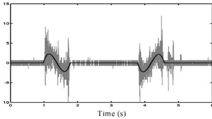
Figure 15. Acceleration and desired acceleration ( m s^{-2} ) versus time.
