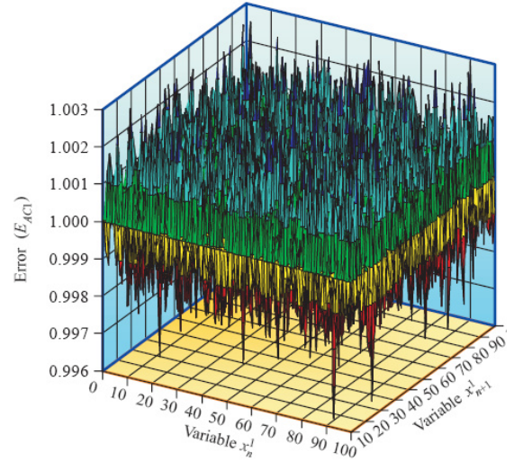
Figure 7. Difference between the autocorrelation distribution function AC_{NSAMPLDISC}(x_n^1, x_{n+1}^1) and the uniform distribution of the 4-coupled symmetric tent map sampled by x^4 for the threshold value 0.998. N_{disc} = 10^2 \times 10^2 , NSampl_{iter} = 10^{10} , \varepsilon_i = i \cdot \varepsilon_1 , \varepsilon_1 = 10^{-14} . Initial values: x_0^1 = 0.330 , x_0^2 = 0.3387564 , x_0^3 = 0.50492331 , x_0^4 = 0.0 .
