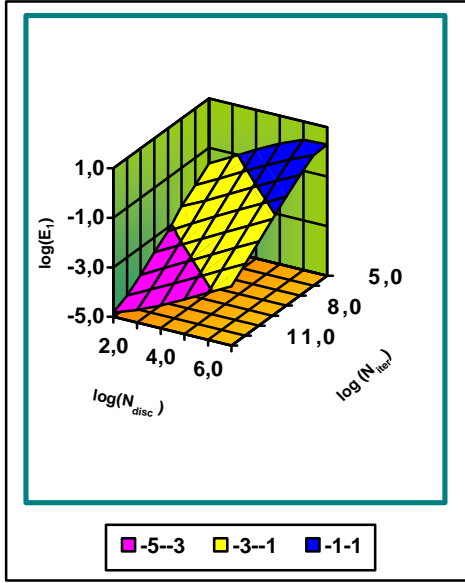
Figure 2. Error E_1 for 3-coupled Symmetric Tent Maps. Computations done using double precision numbers ( \sim 14 - 15 digits) with respect to both N_{\text{iter}} and N_{\text{disc}} , \varepsilon_i = i \cdot \varepsilon_1 , \varepsilon_1 = 10^{-14} , N_{\text{iter}} = 10^5 to 10^{12} , N_{\text{disc}} = 10^2 to 10^7 . Initial values x_0^1 = 0.330000013113 , x_0^2 = 0.338756413113 , x_0^3 = 0.331353442113 , x_0^4 = 0.333213583113 .
