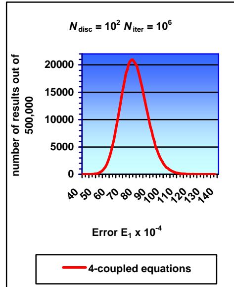
Figure 3. Distribution of the error E_1 for 500,000 initial values for 4-coupled symmetric tent maps.
