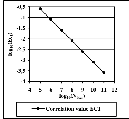
Figure 4. Error E_{C1} for the first and the second components (x^1, x^2) of the 4-coupled symmetric tent map. N_{disc} is fixed to 10^2 \times 10^2 , \varepsilon_i = i \cdot \varepsilon_1 , \varepsilon_1 = 10^{-14} , N_{iter} varies from 10^5 to 10^{11} . Computations are done using double precision numbers ( \sim 14-15 digits). x_0^1 = 0.330 , x_0^2 = 0.3387564 , x_0^3 = 0.50492331 , x_0^4 = 0.0 .
