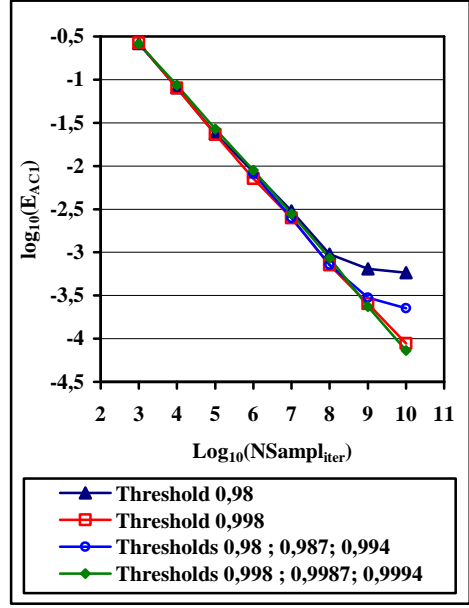
Figure 9. Error of E_{AC1}(N_{disc}, NSampl_{iter}) N_{disc}=10^2 \times 10^2, NSampl_{iter}=10^3 to 10^{10}, \varepsilon_i = i \cdot \varepsilon_1, \varepsilon_1=10^{-14} .
