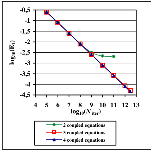
Figure 1. Error E_1 for 2, 3 and 4-coupled Symmetric Tent Maps. Computations done using double precision numbers ( \sim 14 - 15 digits), \varepsilon_i = i \cdot \varepsilon_1 , \varepsilon_1 = 10^{-14} , N_{disc} = 10^4 . Initial values x_0^1 = 0.330000013113 , x_0^2 = 0.338756413113 , x_0^3 = 0.331353442113 , x_0^4 = 0.333213583113 .
