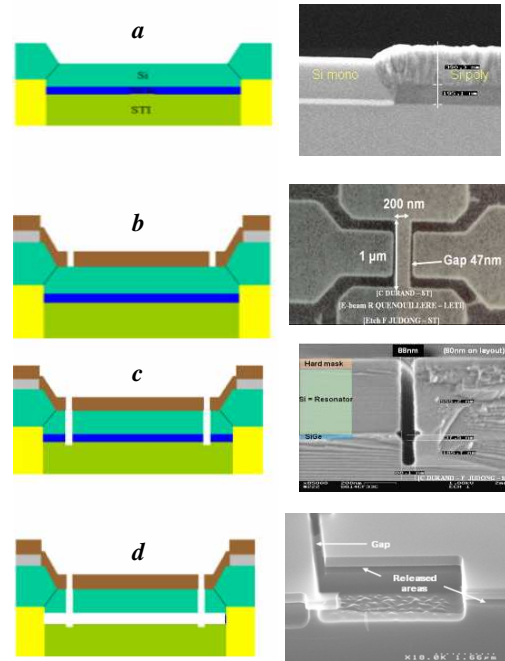
Figure 7: STMicronics SON process
