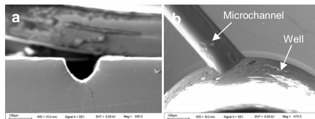
Fig. 3 Scanning electron micrographs of laser cut microchannels on PMMA.
