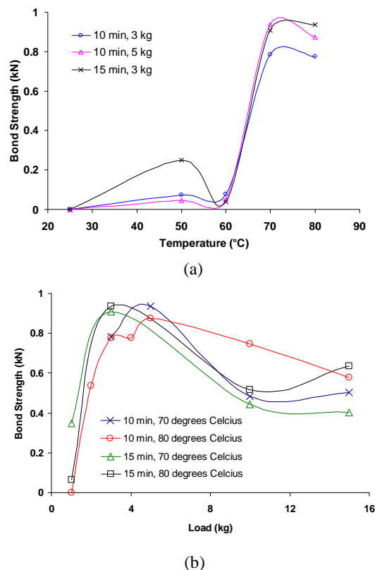
Fig. 5 Results of lap shear test.
