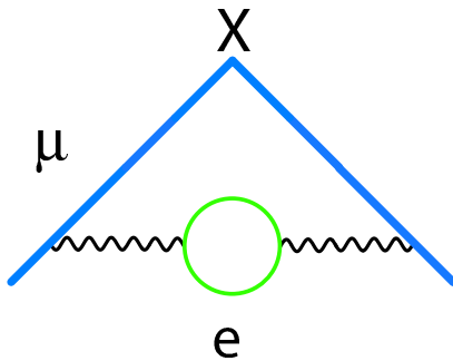
Fig. 3 Fourth-order Feynman diagram with a lowest order vacuum polarization electron-loop.
