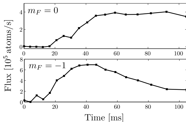
Fig. 4: Flux of atom laser versus time for the guided atom lasers depicted in fig. 1(b), in the m_F = 0 and m_F = -1 spin states (a binning procedure has been used to smooth out the noise due to the CCD camera).
