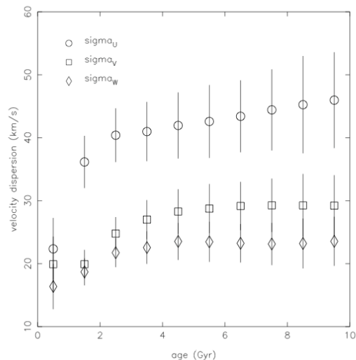
Fig. 14. Age - velocity relations of distant clump giants, with the most probable thick disk, Hercules stream and halo stars being excluded.
