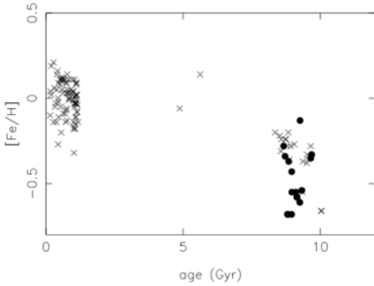
Fig. 10. Age - metallicity diagram for stars with relative age errors lower than 25 % and belonging to the thin disk (crosses) and the thick disk (filled circles).
