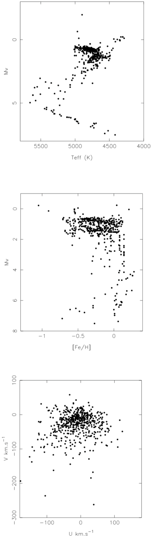
Fig. 8. The NGP sample in the M_v vs T_{\text{eff}} , M_v vs [\text{Fe}/\text{H}] and V vs U diagrams.
