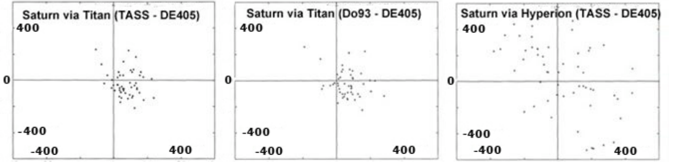
Fig. 5. Residuals (O-C) in \alpha vs \delta on the positions of Saturn deduced from the observed positions of the satellites (a: from Titan TASS theory; b: from Titan Do93 theory; c: from Hyperion TASS theory).
