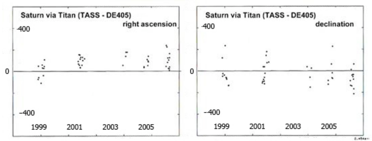
Fig. 4. Residuals (O-C) vs time on the positions of Saturn deduced from the observed positions of Titan.
