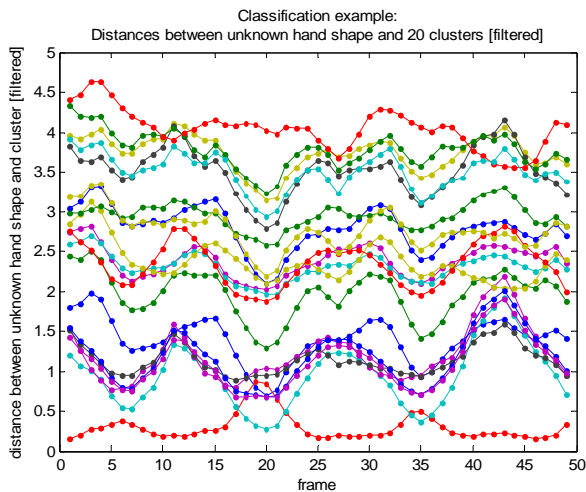
Fig. 9 Classification example: distances between an unknown hand shape and center of 20 clusters (filtered).
