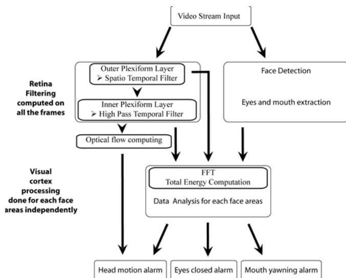
Figure 2: Algorithm for hypo-vigilance features extraction from video data
