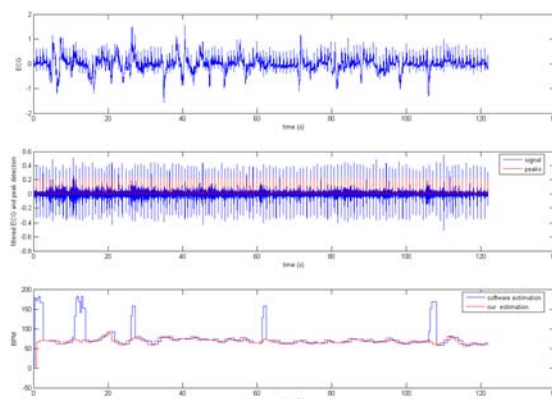
Figure 8: ECG before (first line) and after pre-filtering (second line); computed heart rate from ECG (third line, red signal)
